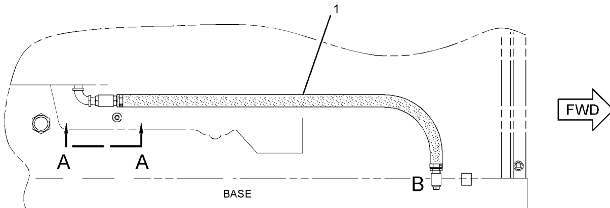
TOP VIEW
